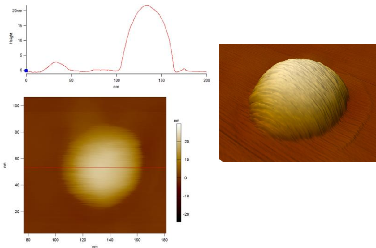
Fig. 5.21 Cross section, respectively, 3D representation of AgCl NPs biosynthesized in the presence of Rhodotorulla Mucilaginosa
