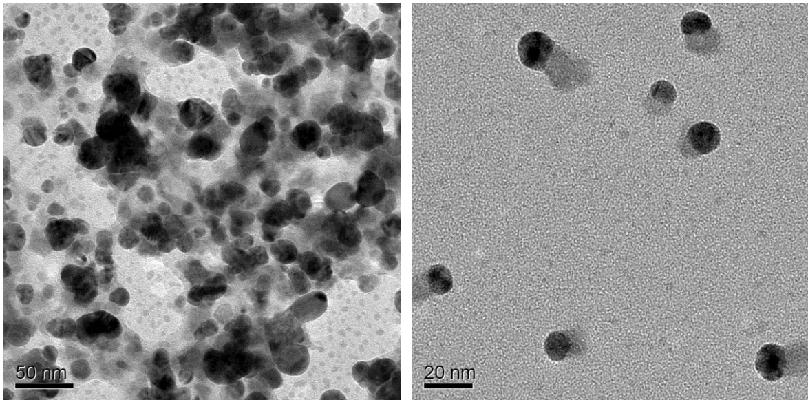
Fig. 5.9 TEM images of nanoparticles synthesized by Raoultella Planticola
