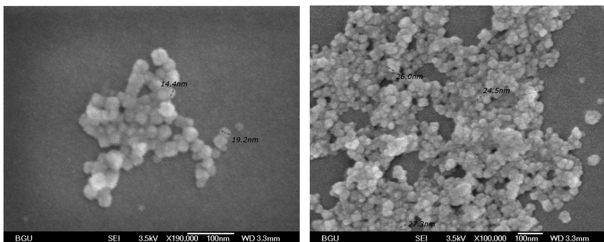
Fig. 5.15 SEM images of nanoparticles synthesized by Rhodotorulla Mucilaginoso and Raoultella Planticola
