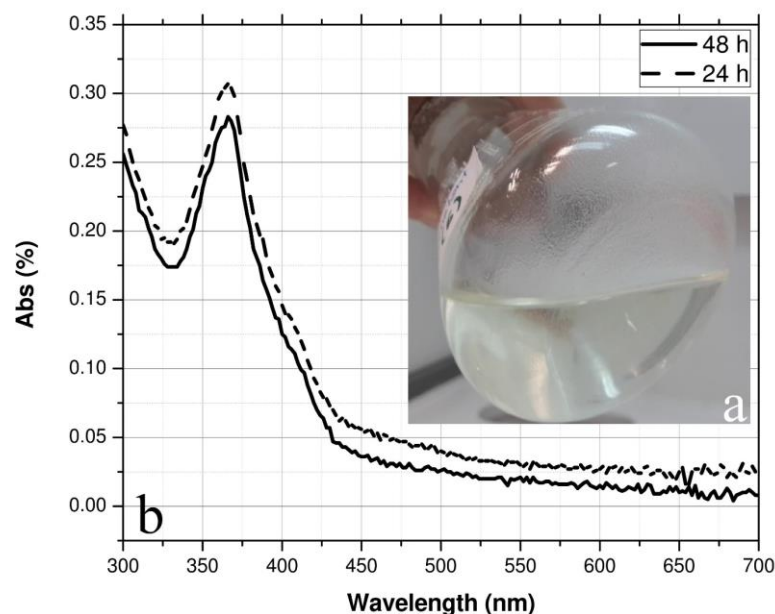
Figure 3.1 UV-vis spectroscopy of synthesized ZnO NPs with peak at 368 nm
