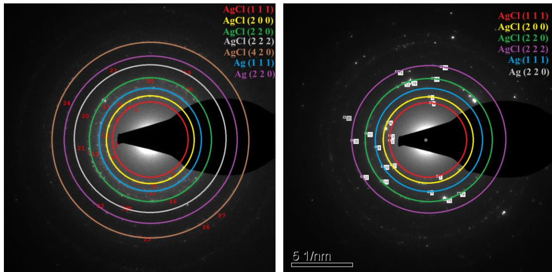
Fig. 5.12 The electron diffraction patterns in the selected area of the AgCl or Ag nanoparticles synthesized in the presence of Rhodotorula Muciluginosa (a) and Raoultella Planticola (b)
