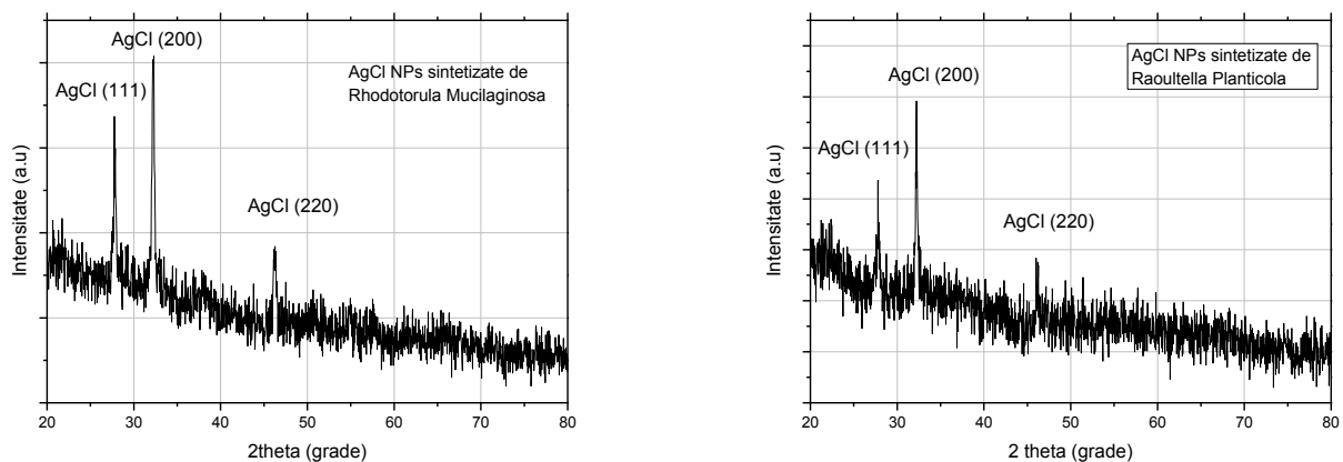
Fig. 5.5 X-ray diffraction spectra for AgCl nanoparticles Rhodotorula Muciluginosa , respectiv Raoultella Planticola
